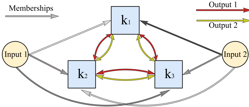
FIGURE II.2: Illustration of the SIMSBM principle — Two input entities are embedded as nodes, linked together by labelled edges. Edges represent the probability of an output given a combination of nodes. Instead of directly modelling such links, we assume a block structure to this network. Nodes belong to clusters to a certain extent, and only the labelled links between these clusters are modelled.
