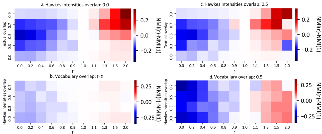
FIGURE IV.12: PDHP performs better than DHP — Difference between the normalized mutual information (NMI) of PDHP and DHP model (Du et al., 2015) for various values of r , intensities overlap and vocabulary overlap, averaged over all the datasets. Red means PDHP performed better, blue means PDHP performed less well. Because \text{PDHP}(r = 1) = \text{DHP} , the column r = 1 show no difference. PDHP allows to increase results on NMI by as much as 0.3 over DHP.
