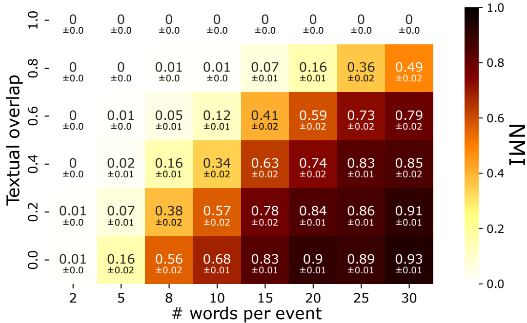
FIGURE IV.26: How much data to use MPDHP — MPDHP performances according to the number of words associated with each event and the overlap between clusters' vocabulary. Overall, MPDHP needs little data. This plot provides a map of how much data must be provided to MPDHP to make it work. For reference, topic overlaps in the real world can be estimated at around 0.25 and the number of named entities per Twitter post around 20.
