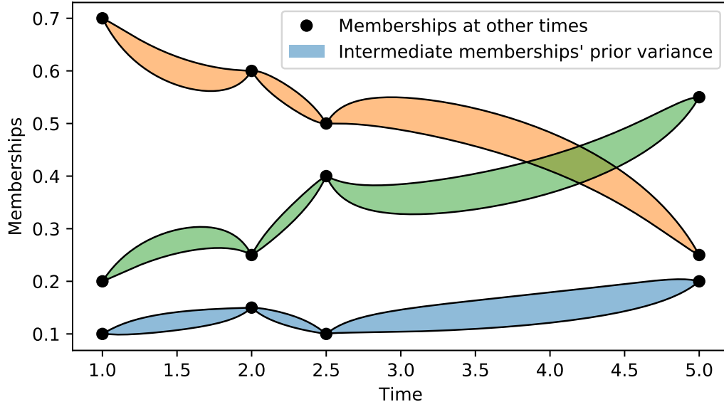
FIGURE II.12: Prior probability's variance on memberships at all times according to the temporal neighbourhood — Variance of the prior over a membership entry (filled curves, we represented 3 such entries as illustration) as a function of time, given some temporal neighbours (black dots). This illustration considers an averaging kernel as \kappa(t, t') = \frac{1}{|t-t'|} . When inferring a parameter x^{(t)} at a time t , the variance of its prior probability P(x^{(t)}) depends on t relative to the temporal neighbours. Here for instance, the variance is null at t = 2 because \kappa(t, t') diverges, and so does \alpha^{(t)} , hence the variance collapsing to 0.
