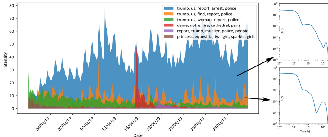
FIGURE IV.20: Limit case of encouraging bursty events clustering — We plot PDHP’s intensity for the News dataset over the observation period for a large value of r . In this case, textual information plays a marginal role, and clusters are inferred based on the events publication dates only.
