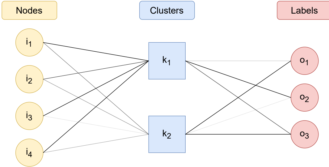
FIGURE II.10: Illustration of the SIMSBM(1), which is the base model coupled to the SDSBM prior. Nodes are associated with clusters, and clusters are associated with labels. Ties between each entity represent a membership and can take values between 0 and 1.
