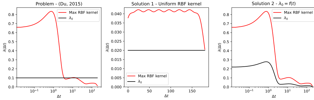
FIGURE IV.22: Choosing the right temporal concentration parameter \lambda_0 — The choice of the temporal concentration parameter \lambda_0 can lead to bias. (Left) The problem with its choice in (Du et al., 2015) is that events happening at large time ranges are likely to go undetected, as the Hawkes intensity at these ranges cannot be larger than \lambda_0 . (Middle) A first solution consists in paving the space with evenly spaced Gaussian functions that all share the same standard deviation. (Right) A second solution is to make \lambda_0 a function of time so that its ratio with the temporal kernel remains constant.
