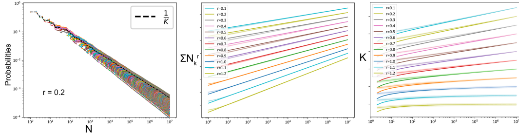
FIGURE IV.4: Numerical validation of Propositions 2 (left), 3 (middle), 4 (right). In the first plot, K is the number of non-empty clusters. In the second and third plots, the theoretical results are the solid lines, and the associated numerical results are the transparent lines of same colour. Except for small N , the difference between theory and experiments is almost indistinguishable.
