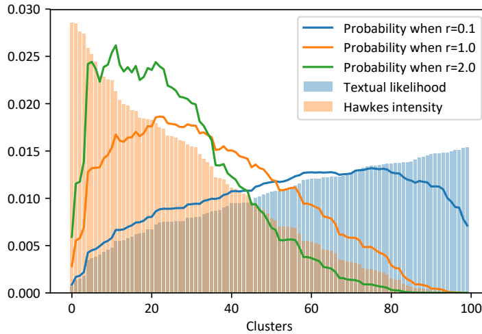
FIGURE IV.9: Effect of r on cluster selection probabilities — The probability for each cluster to get chosen (solid lines) for several values of r and fixed individual textual likelihood (blue bars) and Hawkes intensity (orange bars).
