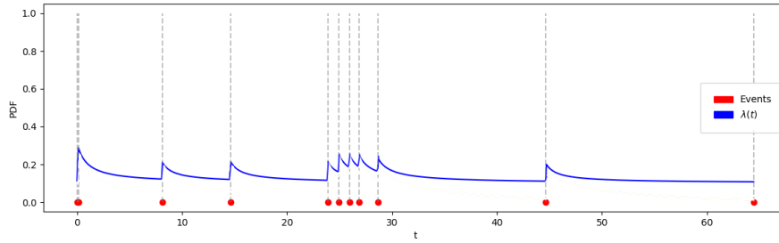
FIGURE IV.2: A realization of a Hawkes process
