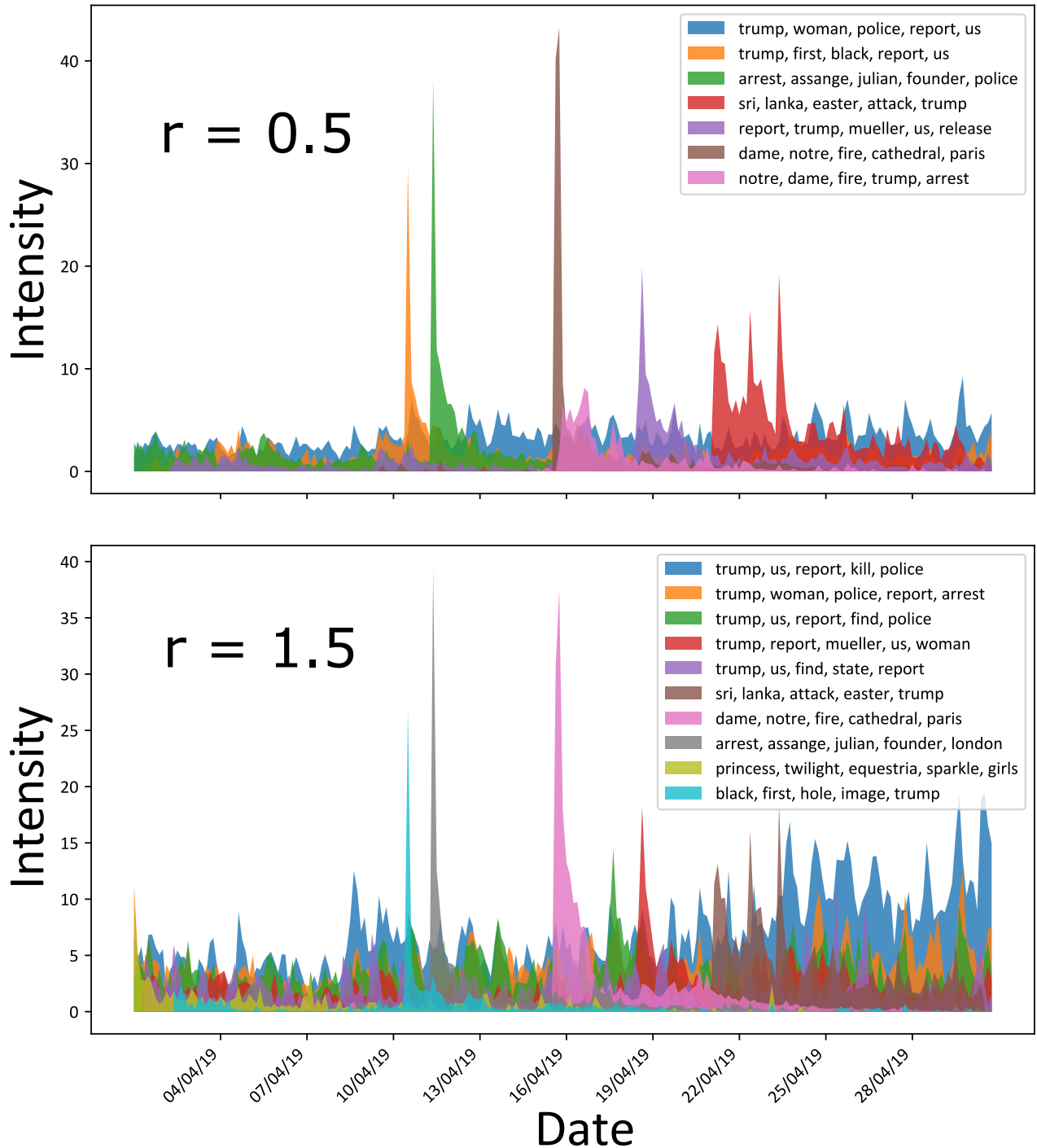
FIGURE IV.19: PDHP allows for modelling bursty events — PDHP’s intensity for the News dataset for two values of r . A lower r finds globally relevant clusters, whereas a higher r allows to recover shorter bursty events.
